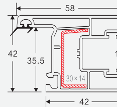
NAME: 88 sliding sash D CODE: 88TLSD WEIGHT(KG/M): 0.84 LENGTH: 5.8-6.0m PCS/BAG: 8 THICKNESS: 2.0
