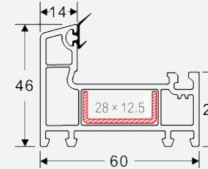
NAME: 60 small frame CODE: 60XX WEIGHT(KG/M): 0.88 LENGTH: 5.9m PCS/BAG: THICKNESS: 2.2
