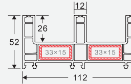
NAME: 112 sliding frame B CODE: 112KB WEIGHT(KG/M): 1.7 LENGTH: 5.8-6.0m
