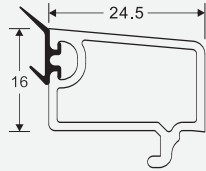
NAME: 88 glazing bead A CODE: 88DYA WEIGHT(KG/M): 0.27 LENGTH: 5.8-6.0m
