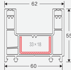
NAME: 60 double sliding frame A CODE: 60LGKA WEIGHT(KG/M): 1.098 LENGTH: 5.8-6.0m
