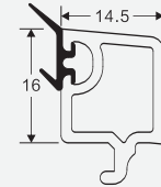
NAME: 88 double glazing bead A CODE: 88SYA WEIGHT(KG/M): 0.18 LENGTH: 5.8-6.0m PCS/BAG: 30 THICKNESS: ②
