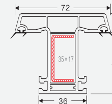
NAME: 60 mullion D CODE: 60ZTD WEIGHT(KG/M): 1.149 LENGTH: 5.8-6.0m
