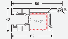
NAME: 60 sliding door sash 3 CODE: 60TLMS3 WEIGHT(KG/M): 1.23 LENGTH: 5.8-6.0m
