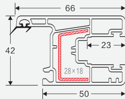
NAME: 88 sliding sash A2 CODE: 88TLSA2 WEIGHT(KG/M): 1.042 LENGTH: 5.8-6.0m
