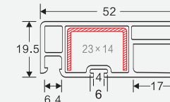
NAME: Screen sash A2 CODE: 52SS2 WEIGHT(KG/M): 0.492 LENGTH: 5.8-6.0m
