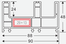
NAME: 90 sliding frame CODE: 90TLK WEIGHT(KG/M): 1.34 LENGTH: 5.8-6.0m
