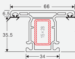
NAME: 42 sash mullion 2 CODE: 42SZT2 WEIGHT(KG/M): 0.84 LENGTH: 5.8-6.0m PCS/BAG: 8 THICKNESS: 2.2
