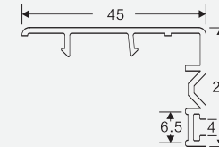
NAME: 88 sliding sash cover CODE: 88FG WEIGHT(KG/M): 0.227 LENGTH: 5.8-6.0m
