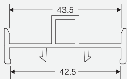
NAME: 42 interlock CODE: 42GM WEIGHT(KG/M): 0.285 LENGTH: 5.8-6.0m PCS/BAG: 20 THICKNESS: 2.2
