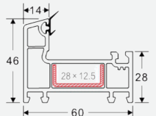
NAME: 60 small frame CODE: 60XX WEIGHT(KG/M): 0.88 LENGTH: 5.9m PCS/BAG: THICKNESS: 2.2
