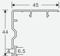
NAME: 60 sliding door sash cover CODE: 60TLMSFG WEIGHT(KG/M): 0.217 LENGTH: 5.8-6.0m
