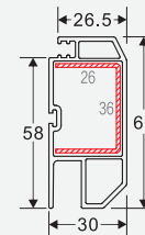
NAME: 66 Screen door sash CODE: SSA3 WEIGHT(KG/M): 0.635 LENGTH: 5.8-6.0m
