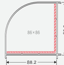
NAME: 88 right angle bay corner adaptor CODE: 88ZJ WEIGHT(KG/M): 0.967 LENGTH: 5.8-6.0m PCS/BAG: 4 THICKNESS: 1.8 ②
