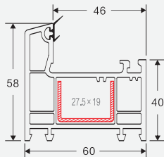
NAME: 60 frame D CODE: 60PKD WEIGHT(KG/M): 1.042 LENGTH: 5.8-6.0m
