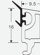
NAME: 88 double glazing bead C CODE: 88SYC WEIGHT(KG/M): 0.15 LENGTH: 5.8-6.0m PCS/BAG: 30 THICKNESS: ②
